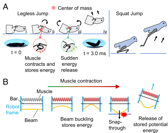
Fig. 1. Bioinspiration and principle of operation of the jumping robot. (A) Click beetles amplify muscle power through morphology to produce extremely fast movements by “clicking” their bodies to generate jumps for hunting and escape, while other insects (e.g., locusts) initiate jumping by the traditional means of jointed appendages. (B) Concept of an insect-scale robot capable of slowly storing elastic energy in buckled beams by the contraction of coiled artificial muscles and the quick release of stored energy by triggering beam snap-through to achieve effective jumping without legs.
